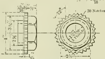
ADJUSTING NUTS ON VALVE STEM AT CROSSHEAD
